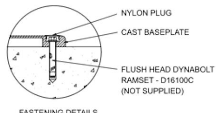
FASTENING DETAILS
